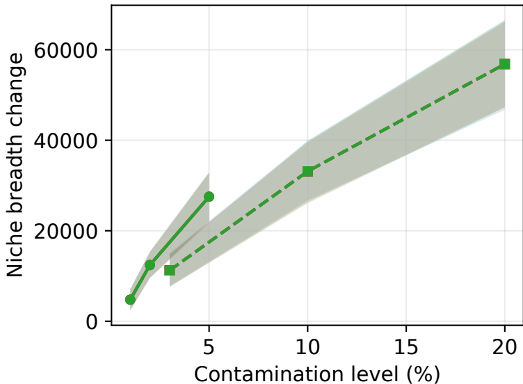
(a) Niche breadth change
