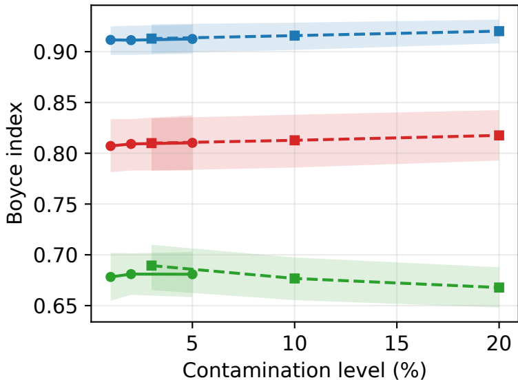
(a) Boyce index
