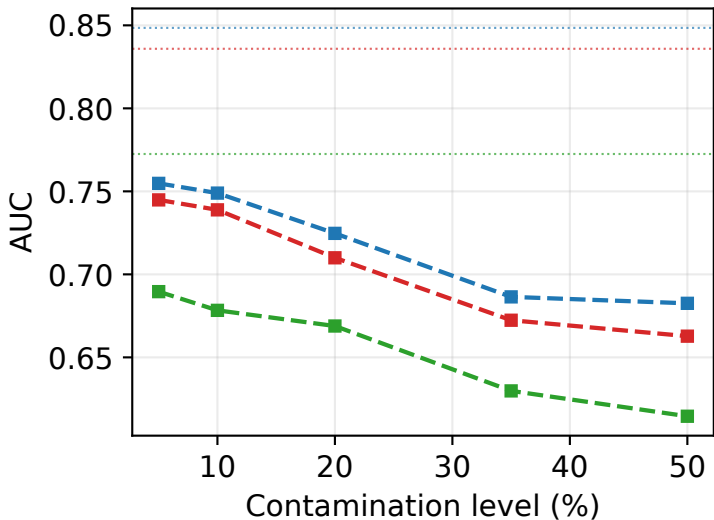
(S9) A. astacus — combined, lowacc
