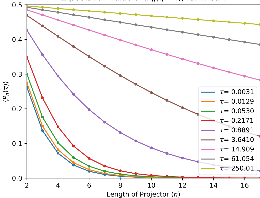
Expectation Value of \langle P_n(t_f = \tau) \rangle for fixed \tau
