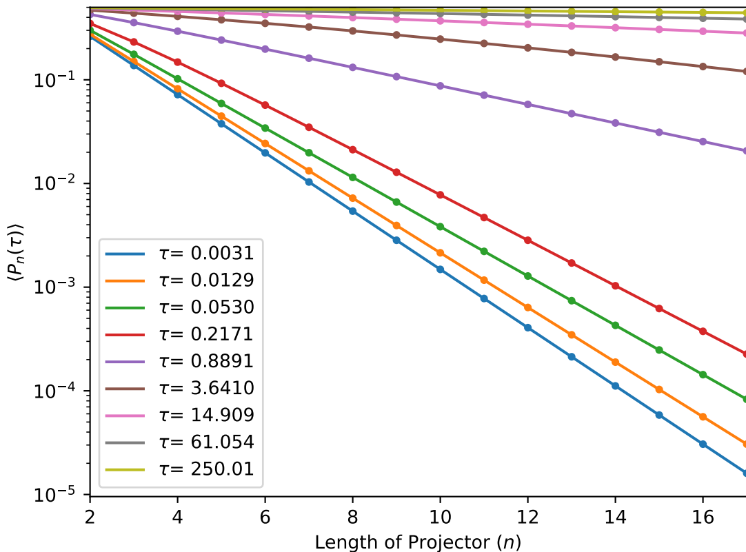
Expectation Value of \langle P_n(t_f = \tau) \rangle for fixed \tau
