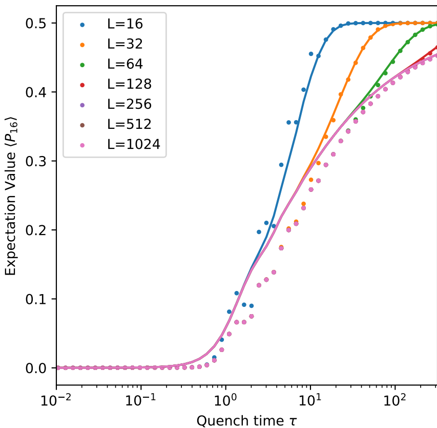
G_1 approximation for P_{16}
