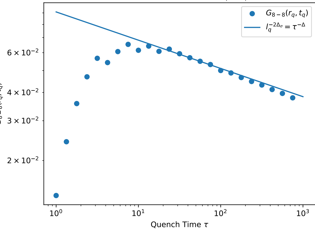
Scale invariant function with r_q = t_q = \sqrt{\tau}
