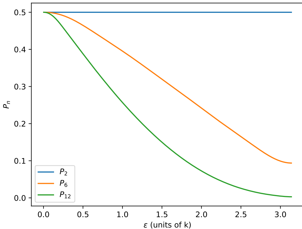
Effect of increasing excluded momentum modes \varepsilon
