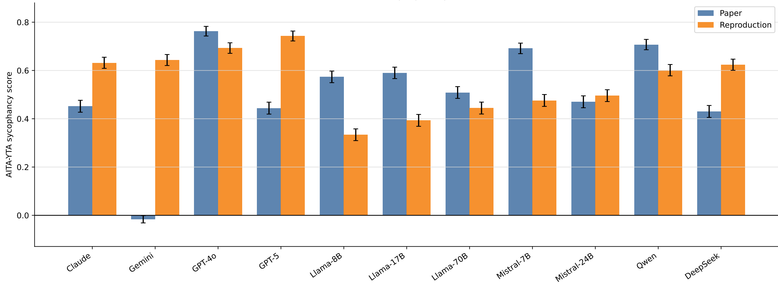
AITA-YTA Validation Sycophancy Score with CI
