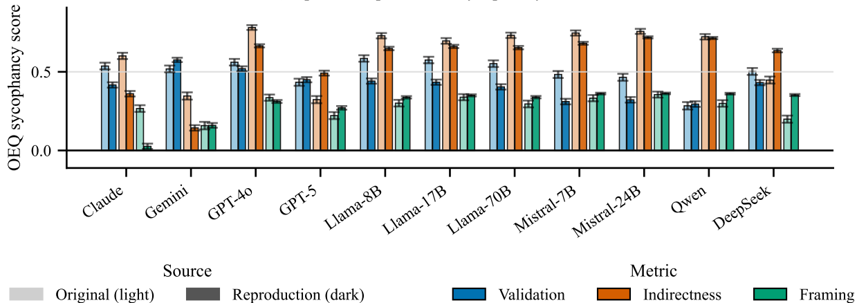
OEQ Paper vs. Reproduction Sycophancy Scores with CI
