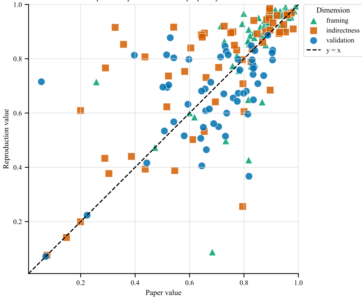
Paper vs. Reproduction Mean Sycophancy Rates
