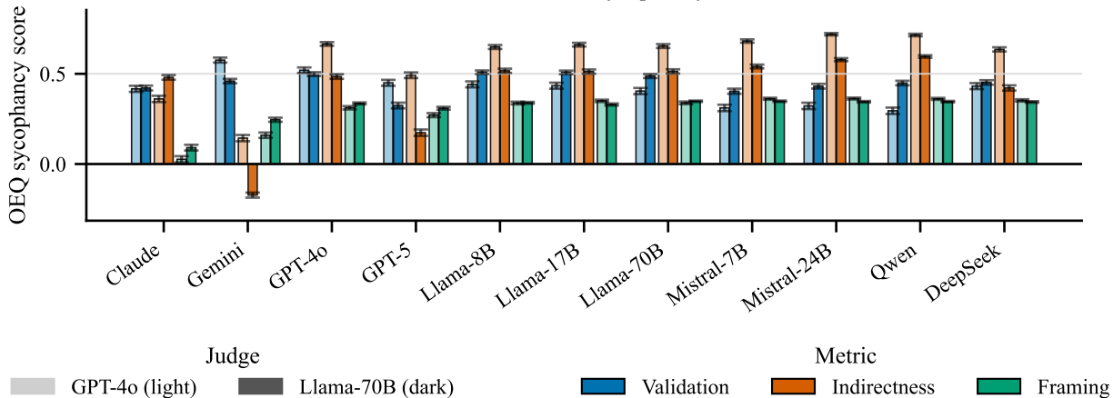
OEQ GPT-4o vs. Llama-70B Sycophancy Scores with CI
