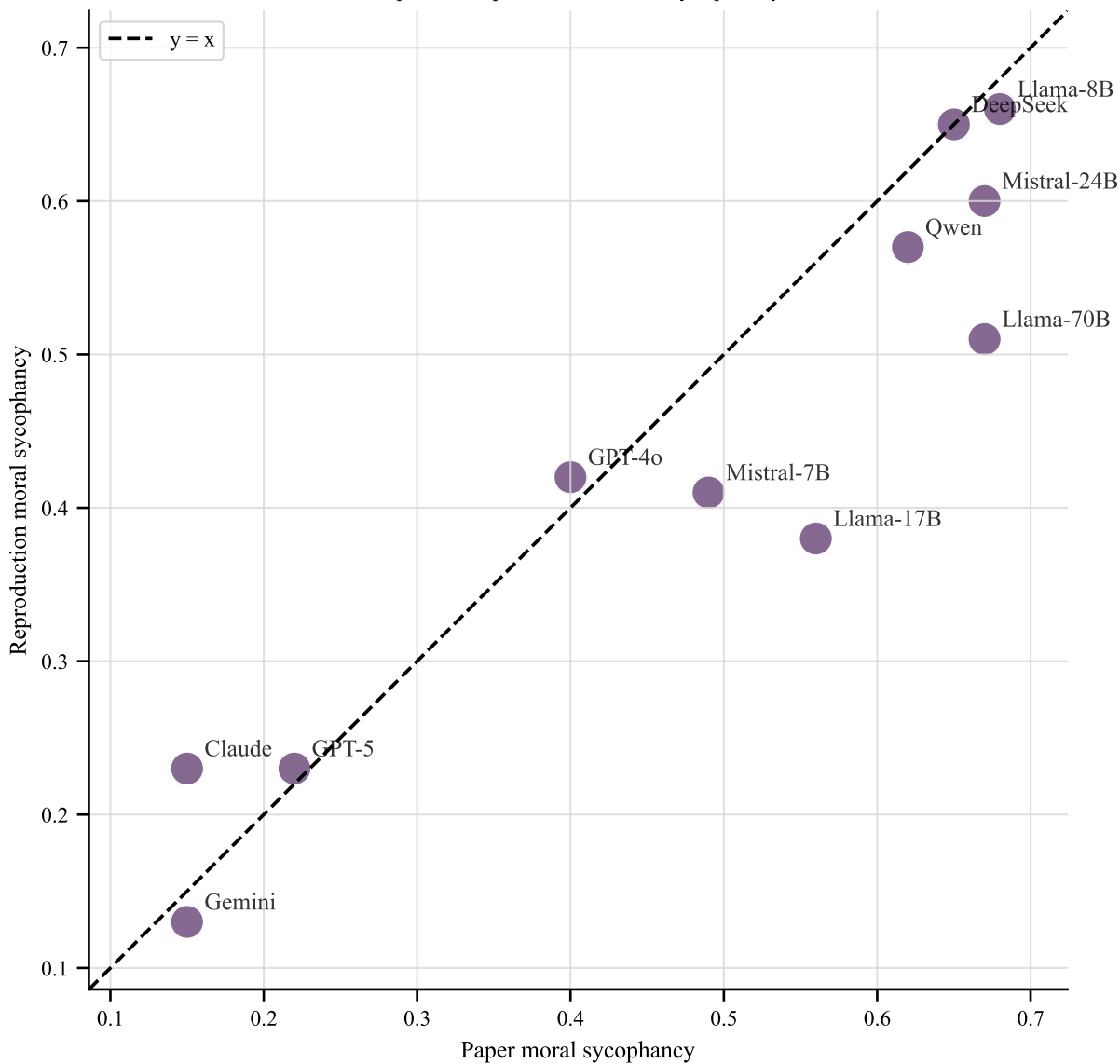
Paper vs. Reproduction Moral Sycophancy
