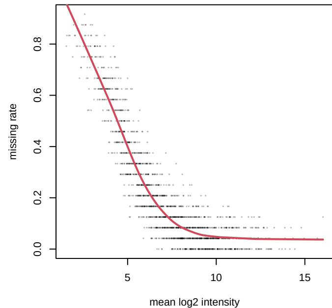
MNAR diagnostic Spearman rho = -0.87
