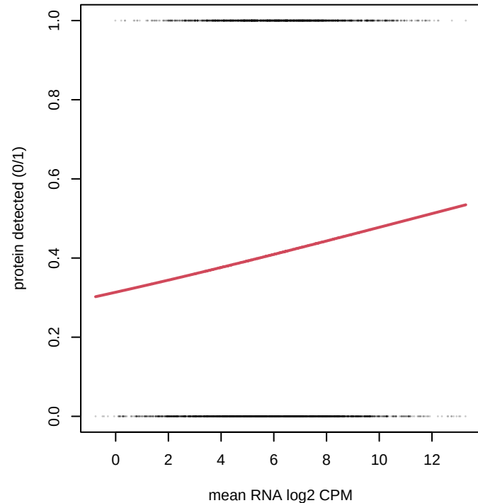
Detectability vs abundance (Tier 2 is mostly a detection limit)
