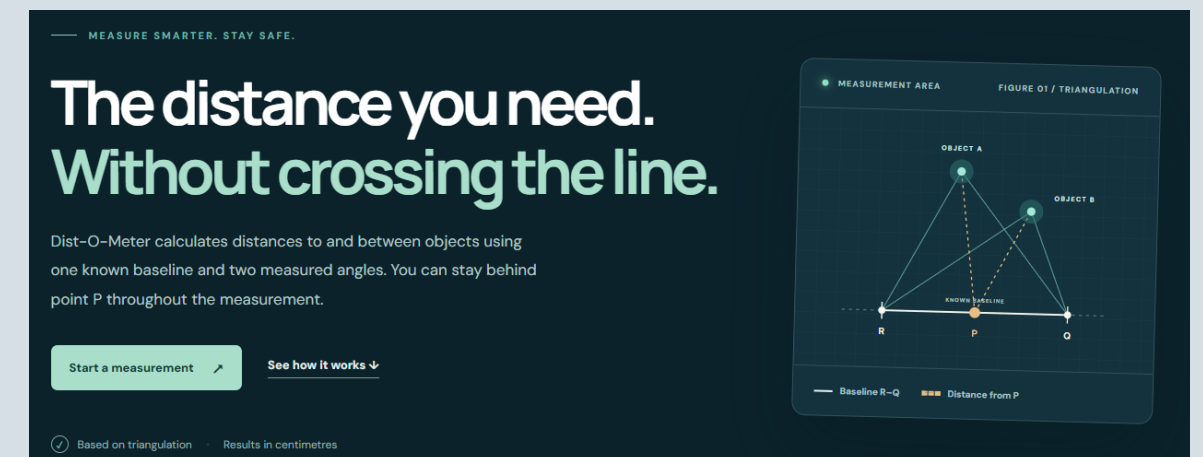
Web application
