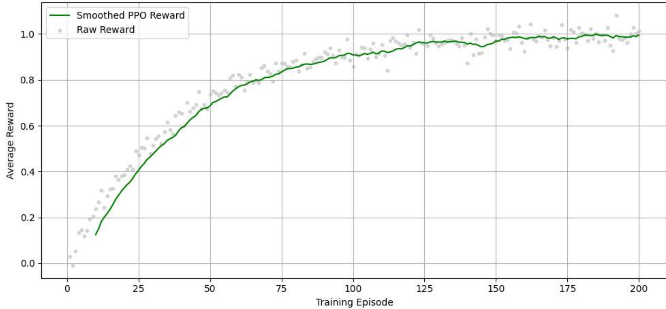
PPO Convergence Curve
