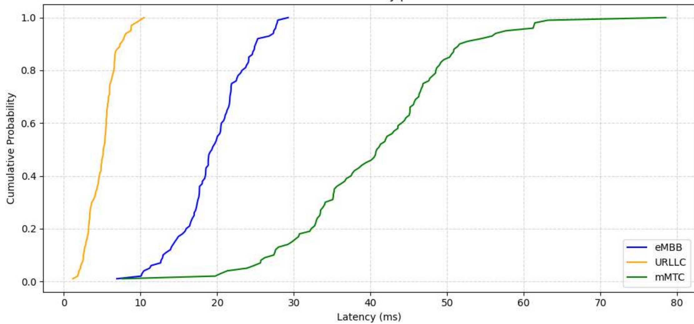
CDF of UE Latency per Slice
