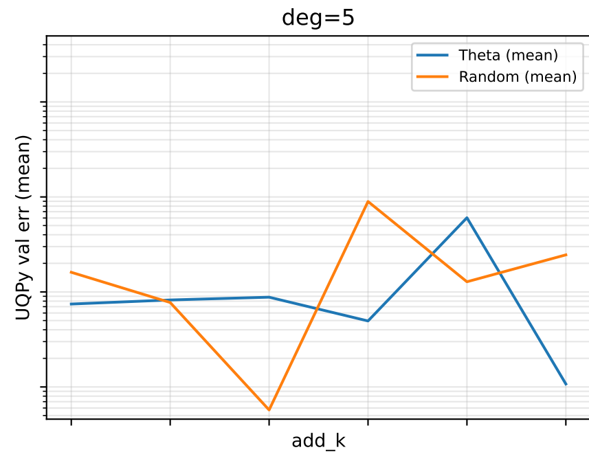
UQPy val err (mean) vs add_k | pocet_start=70
