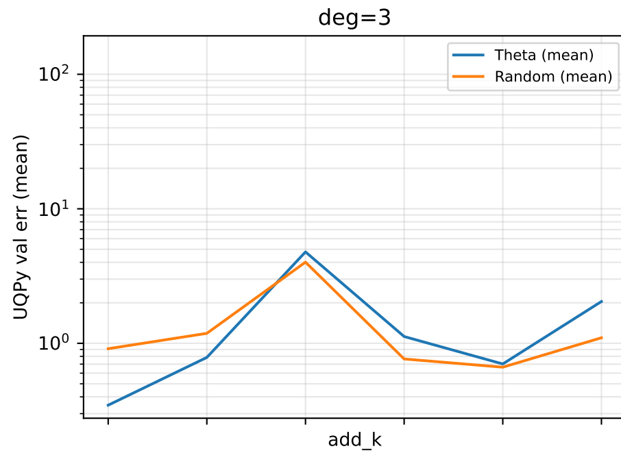
UQPy val err (mean) vs add_k | pocet_start=30
