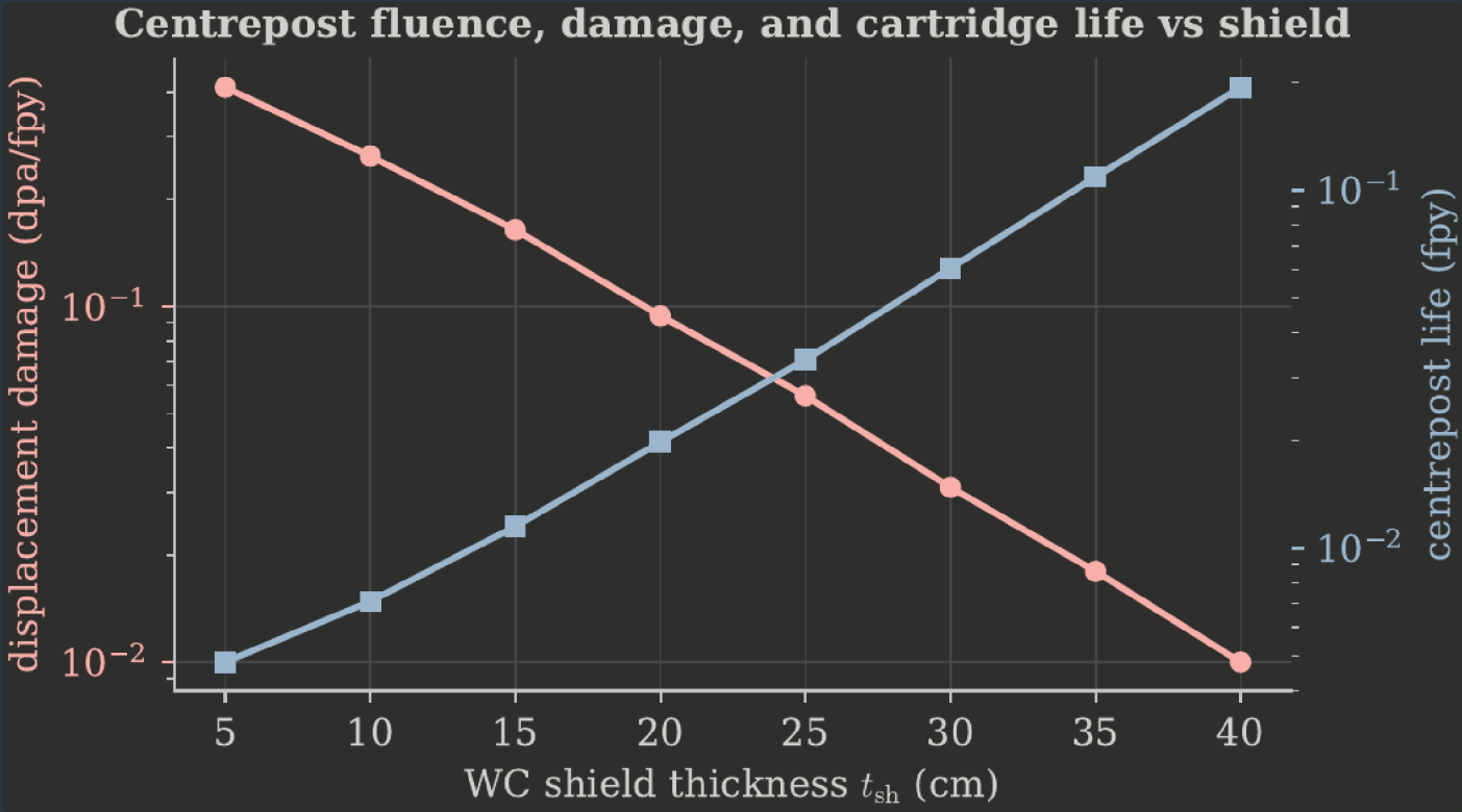
FIGURE 1. Centrepost damage rate and cartridge life versus tungsten-carbide shield thickness. RECOMPUTED
