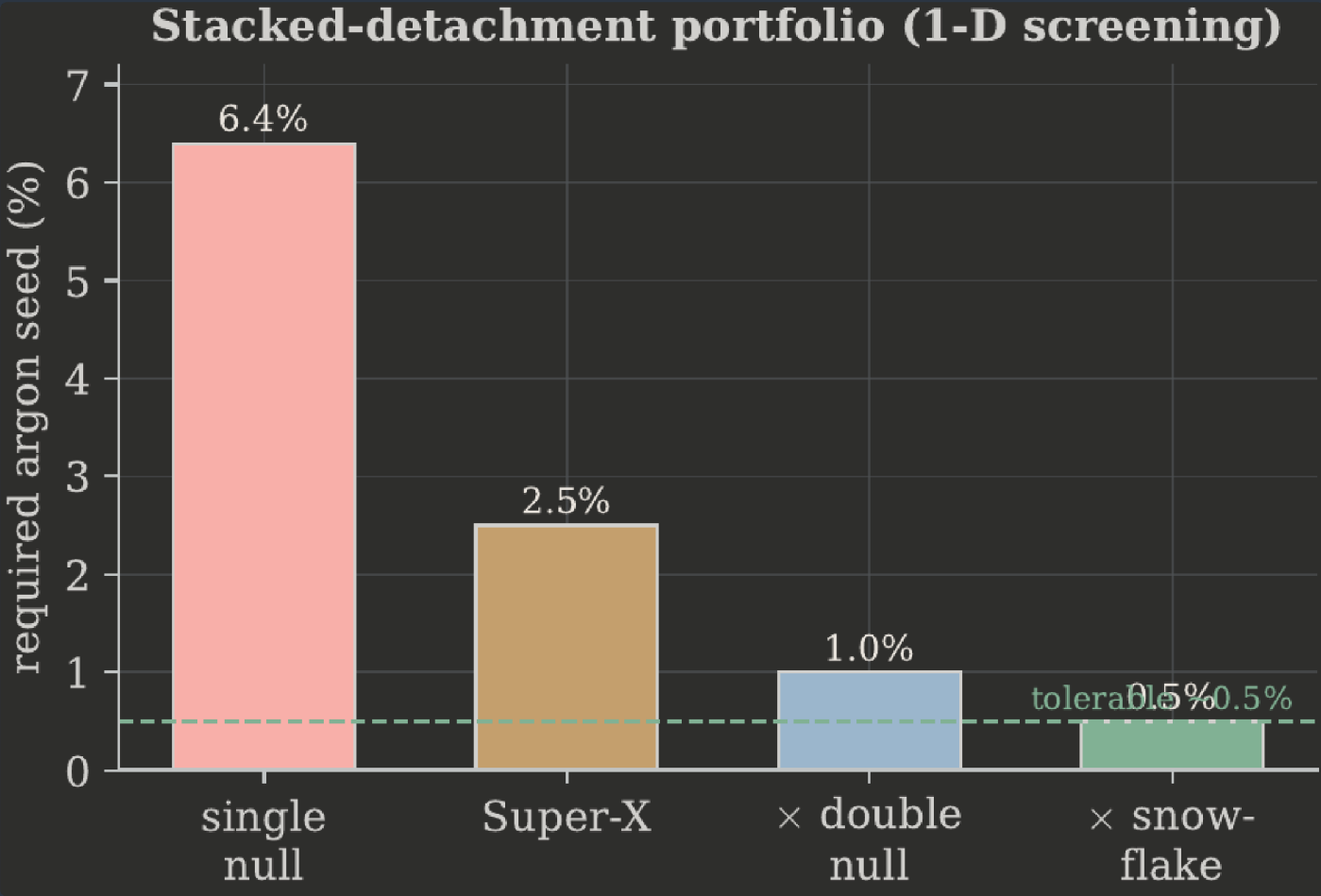
FIGURE 1. Divertor options ranked on detachment against the compact machine’s exhaust load. RECOMPUTED
