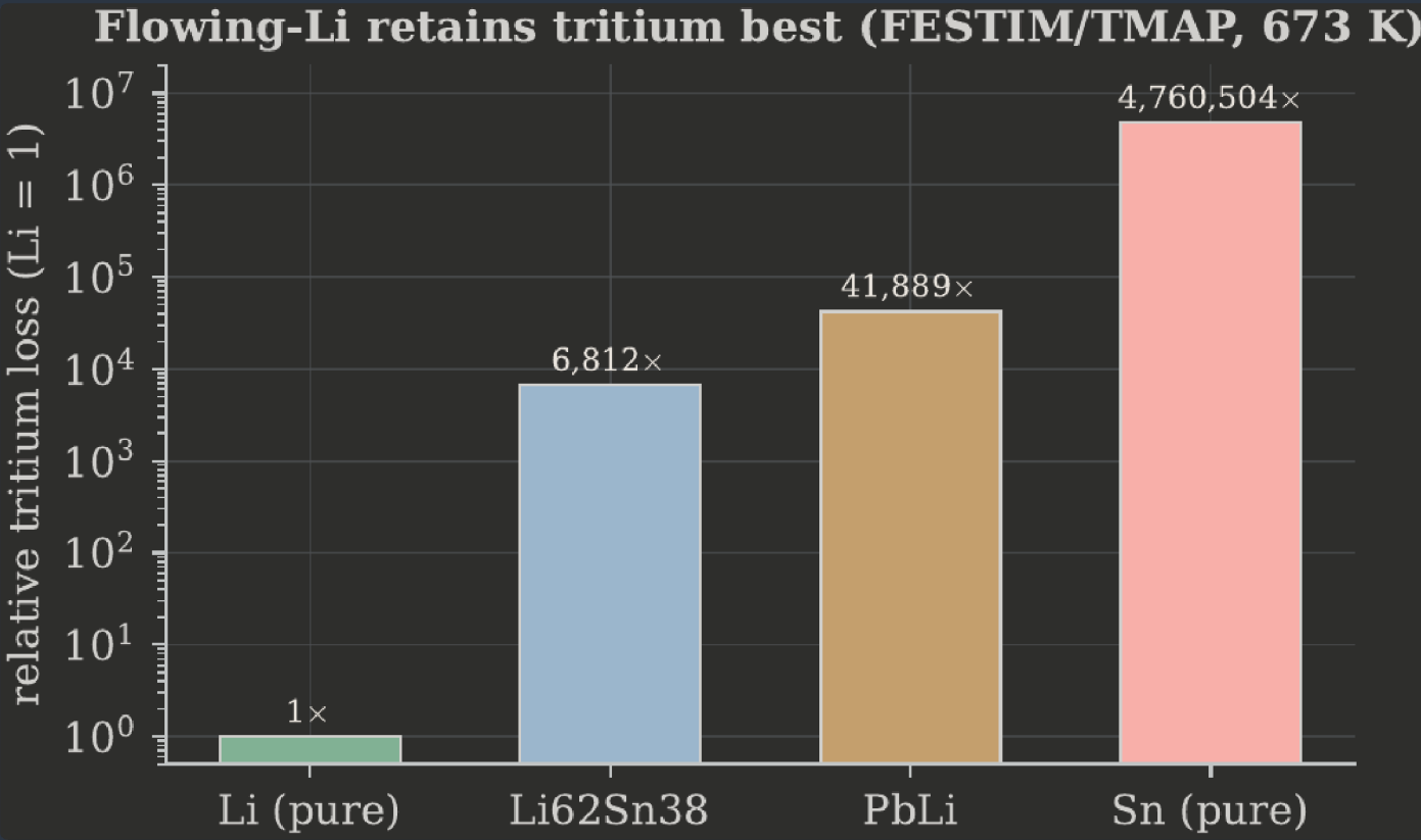
FIGURE 1. Relative tritium loss of four liquid-metal divertor candidates: flowing lithium is optimal. FESTIM/TMAP
