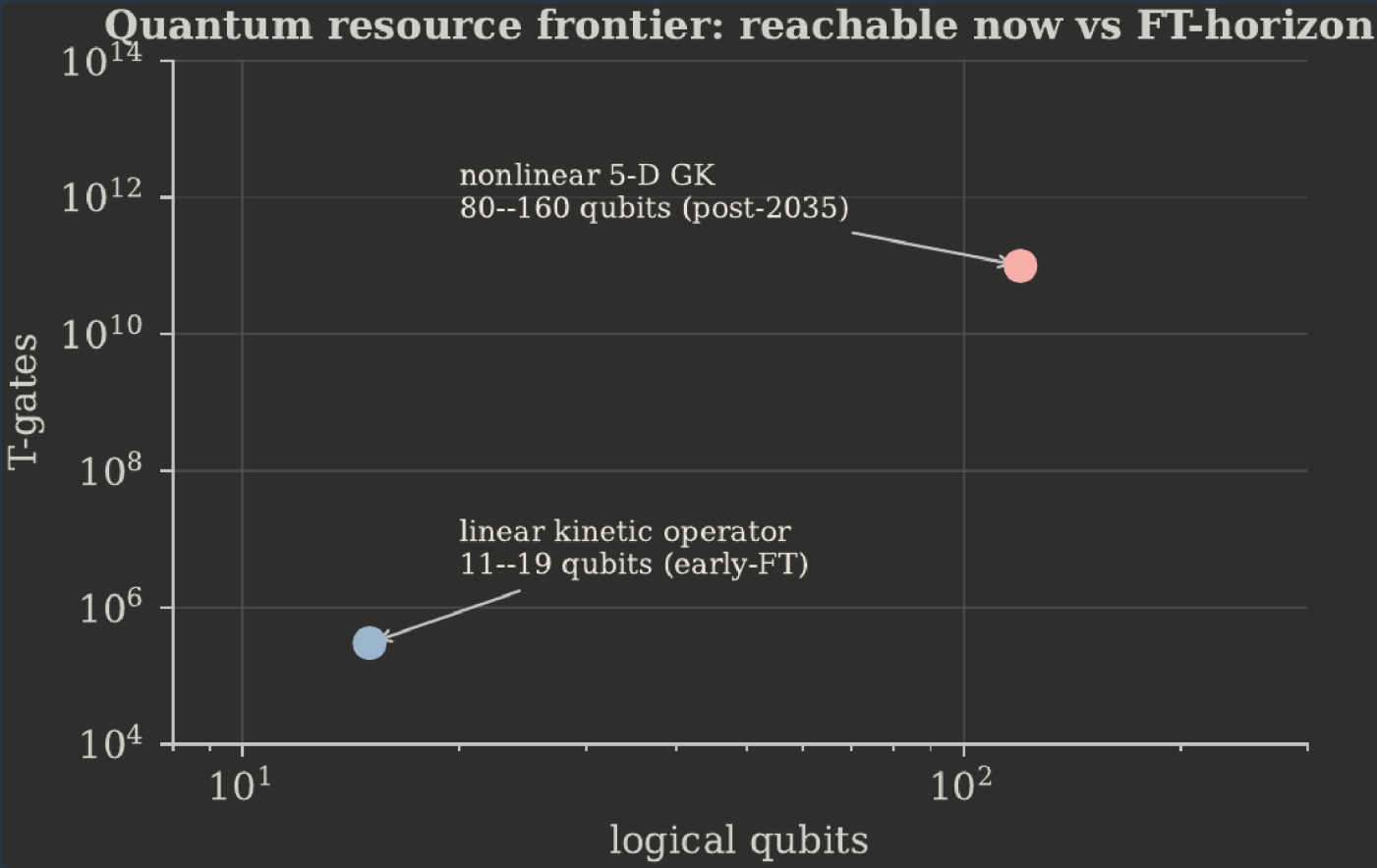
FIGURE 1. The quantum resource frontier: tractable linear operator versus fault-tolerant-horizon gyrokinetics. RESOURCE ESTIMATE
