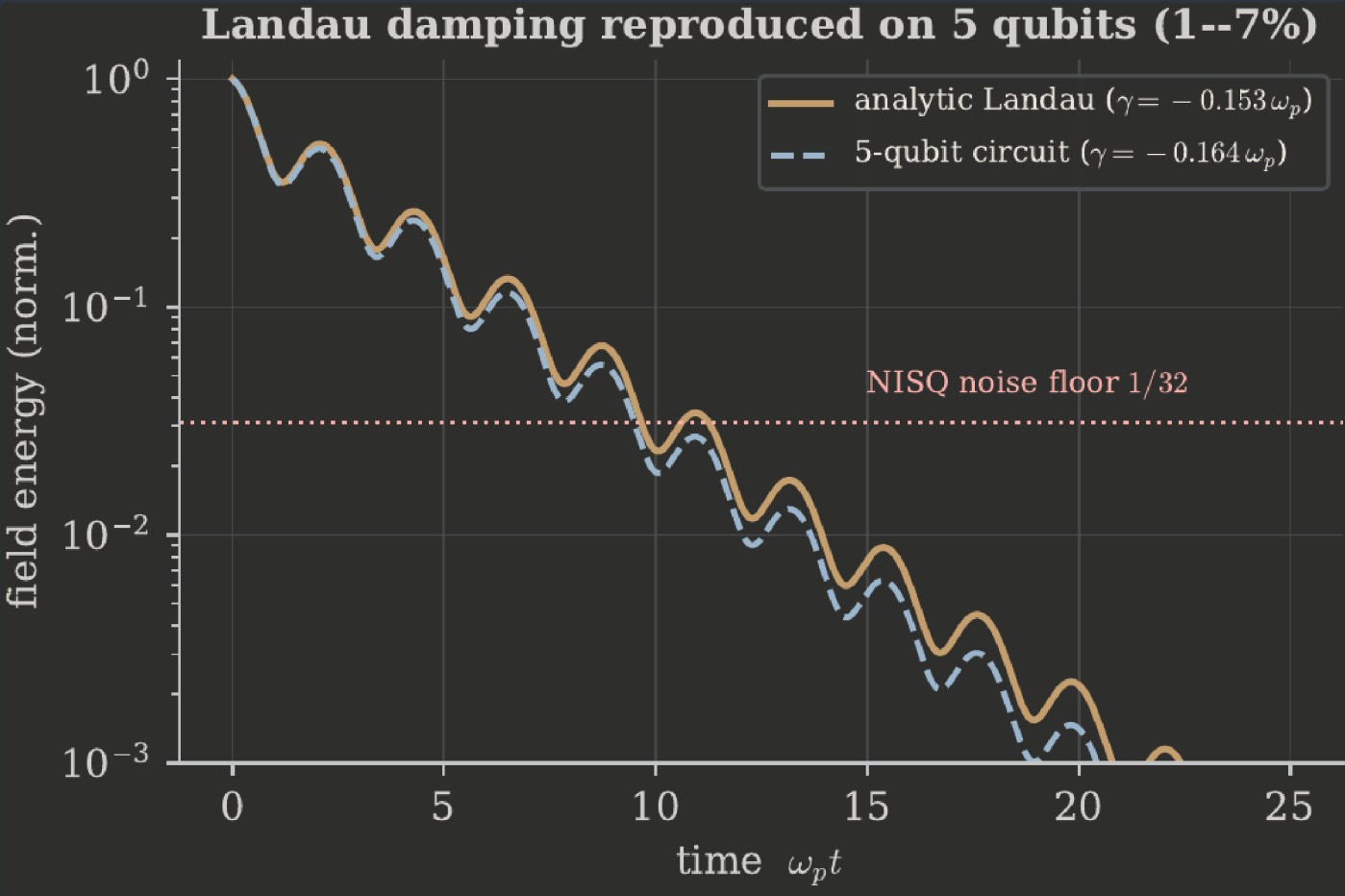
FIGURE 2. Landau damping reproduced on a 5-qubit Hamiltonian-simulation circuit.
