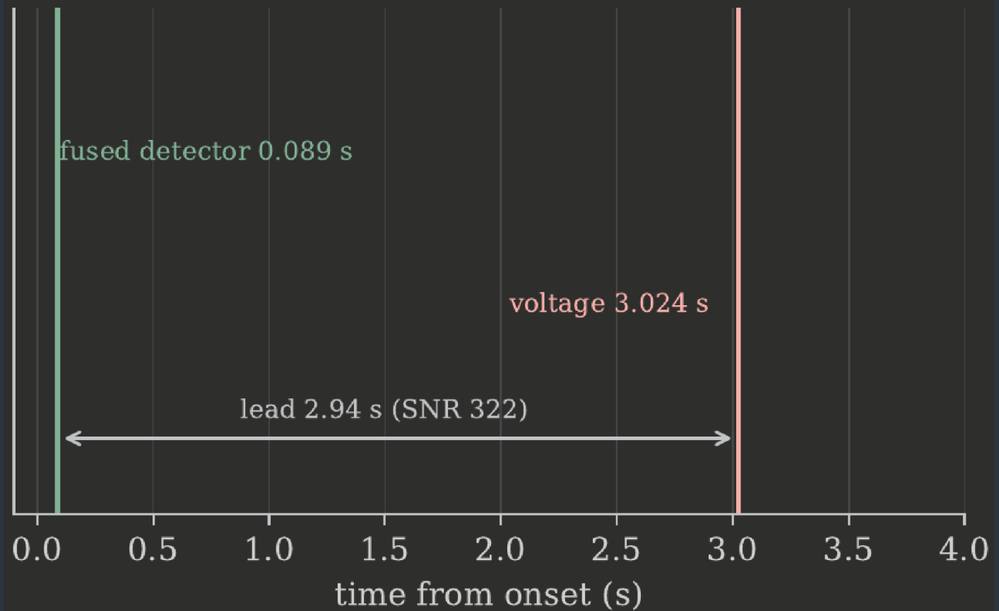
FIGURE 1. Fused strain-rate + magnetization detection fires well ahead of the voltage threshold.
