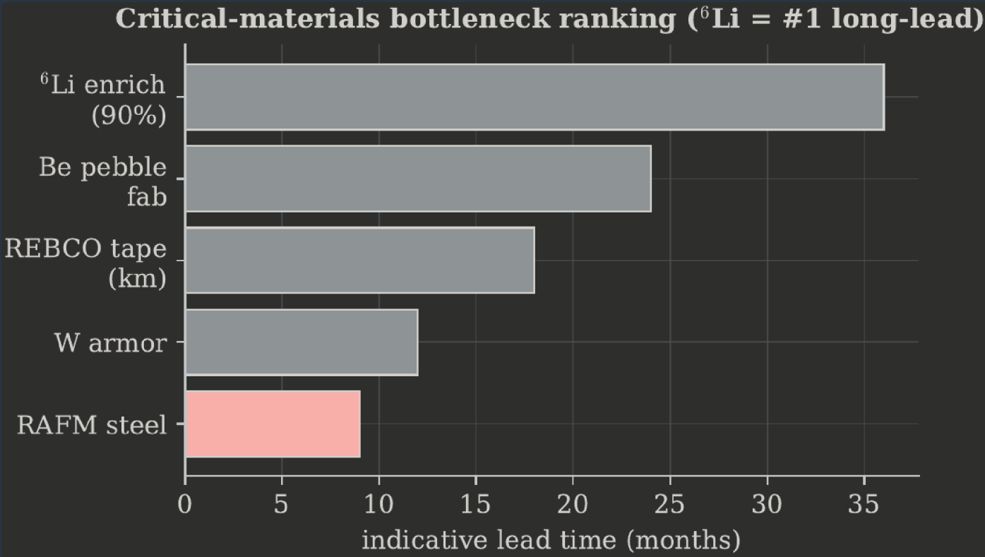
FIGURE 1. Critical-materials lead-time bottleneck ranking; enriched lithium-6 is the binding long-lead item (gate SC-BR-1). BOM
