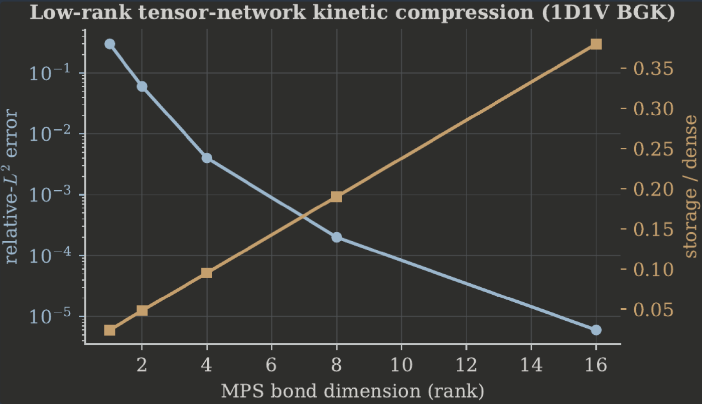
FIGURE 1. Low-rank tensor-network compression of the BGK distribution: exponential error decay and storage vs bond dimension (gate KX-L1-A16). MPS / SVD
