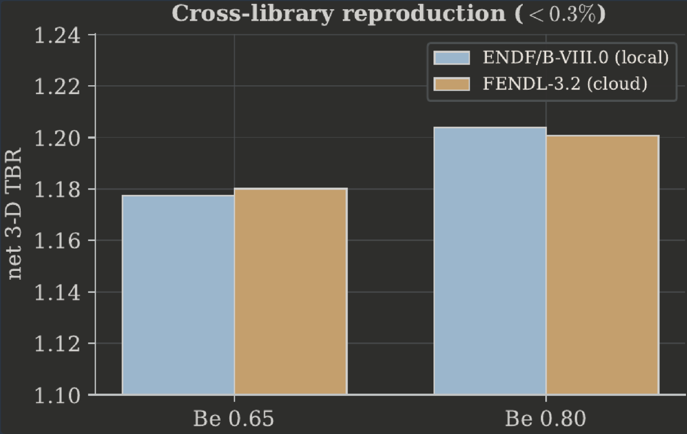
FIGURE 1. The load-bearing TBR reproduced across independent nuclear-data libraries to under 0.3%. CROSS-LIBRARY
