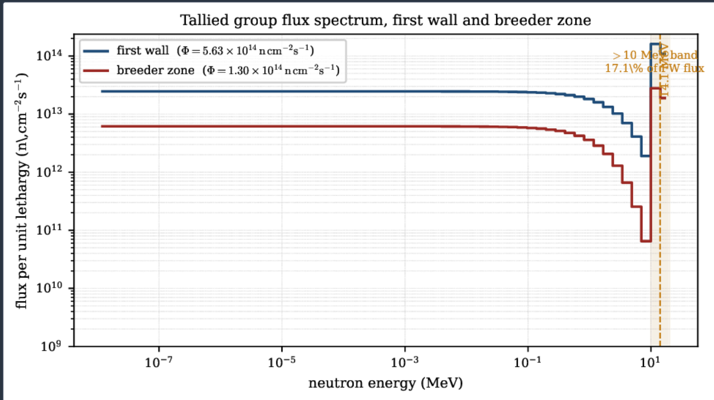
Tallied 175-group neutron flux spectrum at the first wall (blue) and in the breeder zone (red), per unit lethargy. The total flux and the 17.1% fraction above 10 MeV are the tallied integral values (serial BR-L2-A23); the 14.1 MeV peak and slowing-down tail are the representative VITAMIN-J spectral shape. (Schematic group shape; integral flux and 14 MeV-band fraction are tallied.)
