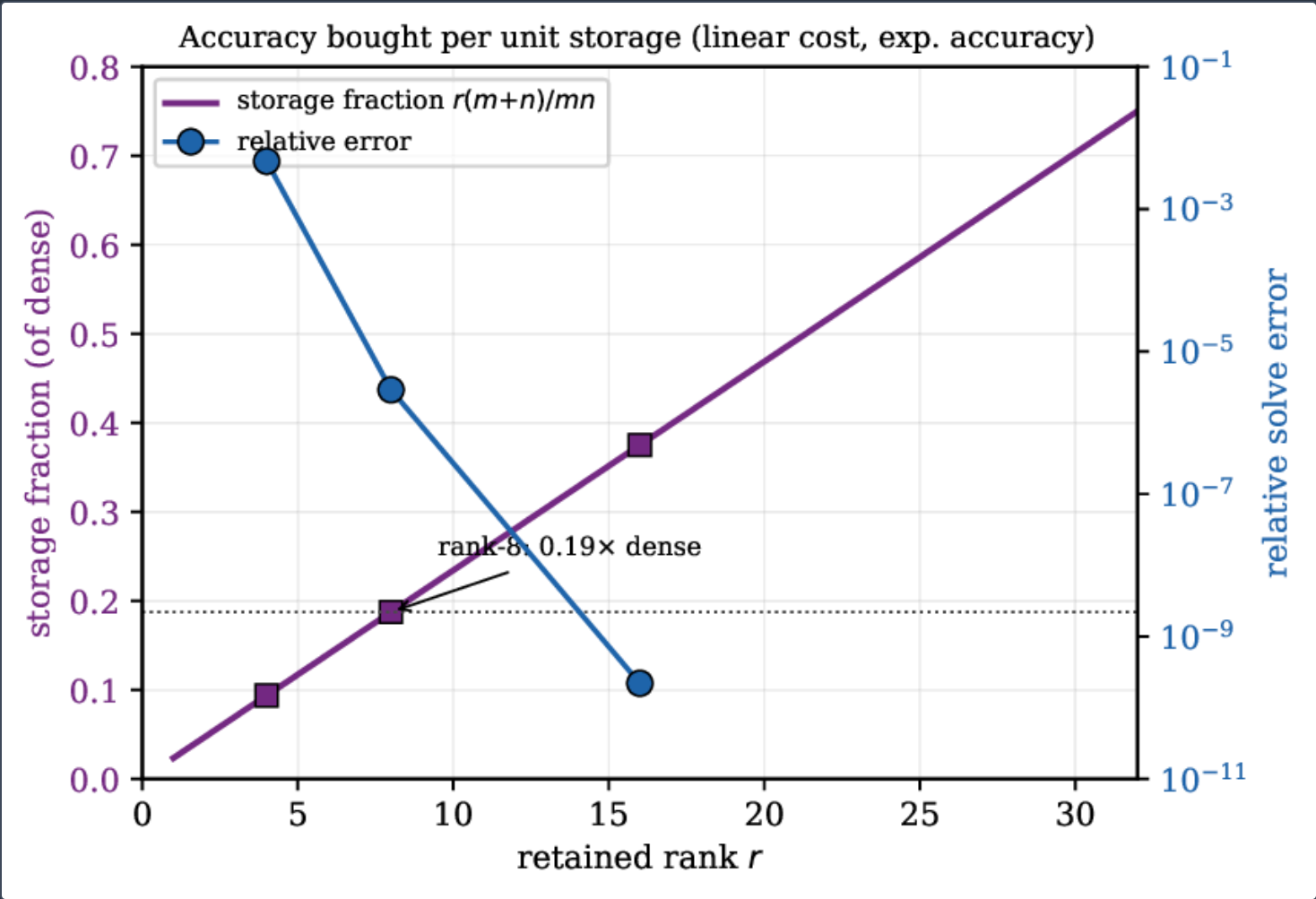
Accuracy bought per unit storage. The low-rank storage fraction \rho_r = r(m+n)/mn grows linearly (rank-8: 0.19x dense, matching equation 12) while the relative solve error falls exponentially — the trade that makes a fast, accurate surrogate possible.
