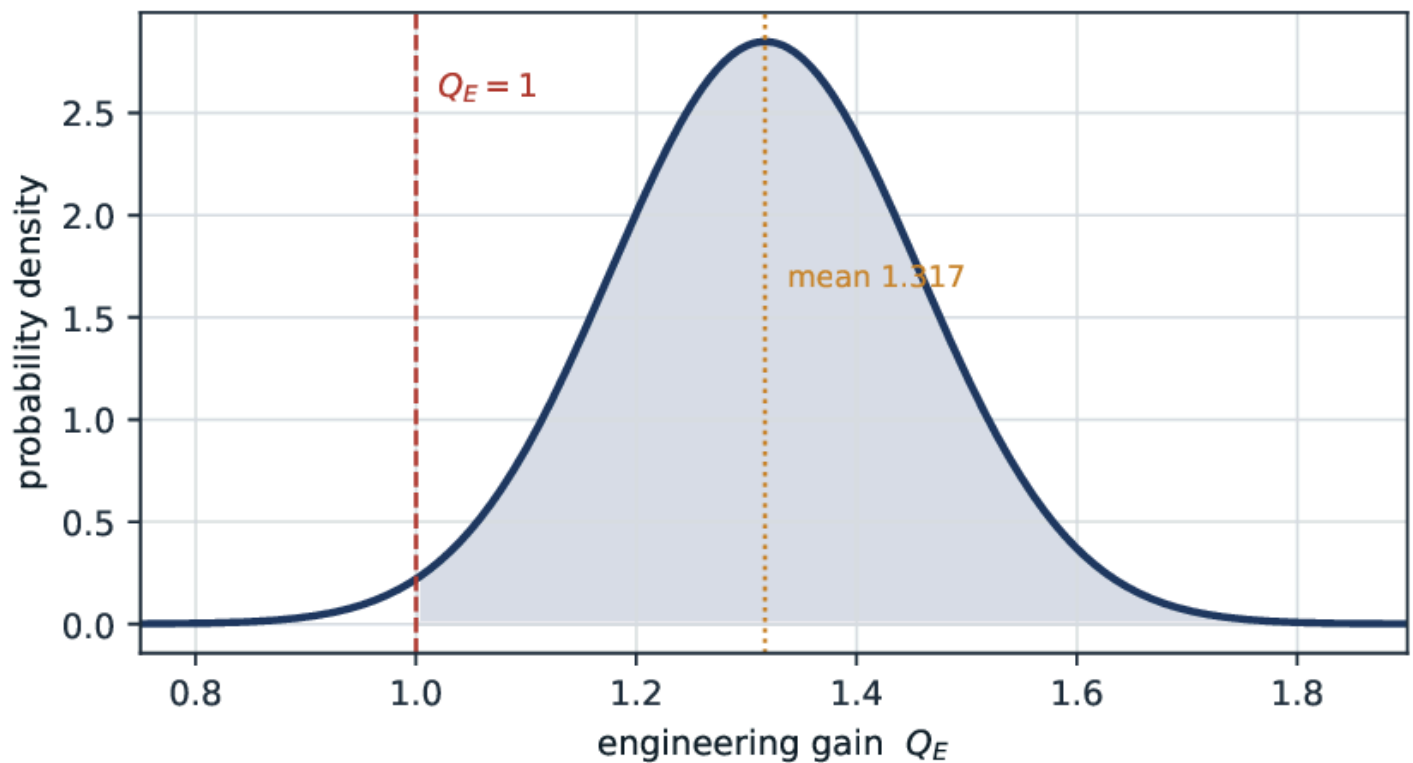
Q E uncertainty over design ranges: P(Q_E > 1) = 1.0 (40\,000 MC)
