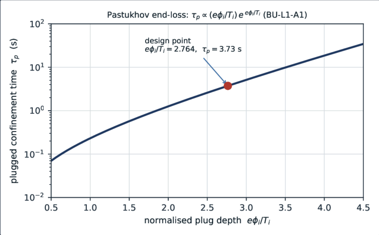
Pastukhov end-loss confinement time \tau_p \propto (e\phi_i/T_i) \exp(e\phi_i/T_i) (BU-L1-A1). The design point at e\phi_i/T_i = 2.764 returns \tau_p = 3.73\text{ s} ; the exponential dependence is the source of the plug's leverage and of its criticality.
