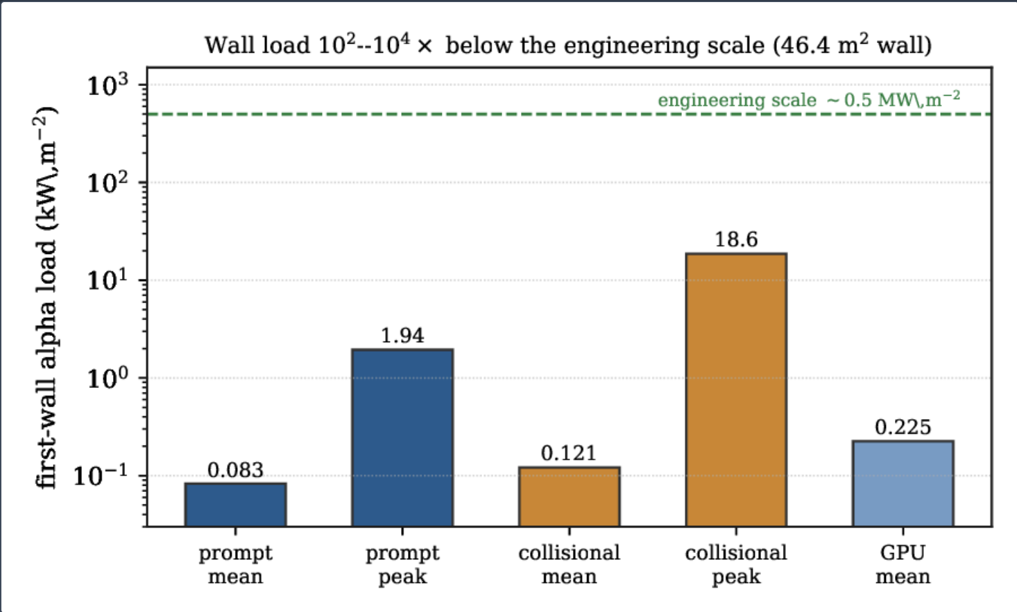
First-wall alpha loads from equation (13) (serial BR-L2-A20), on a logarithmic axis. Prompt and collisional mean/peak loads, and the GPU-follower mean, all sit far below the \sim 0.5 \text{ MW}/\text{m}^2 engineering scale (green dashed). The compact wall ( 46.4 \text{ m}^2 ) is the conservative denominator.
