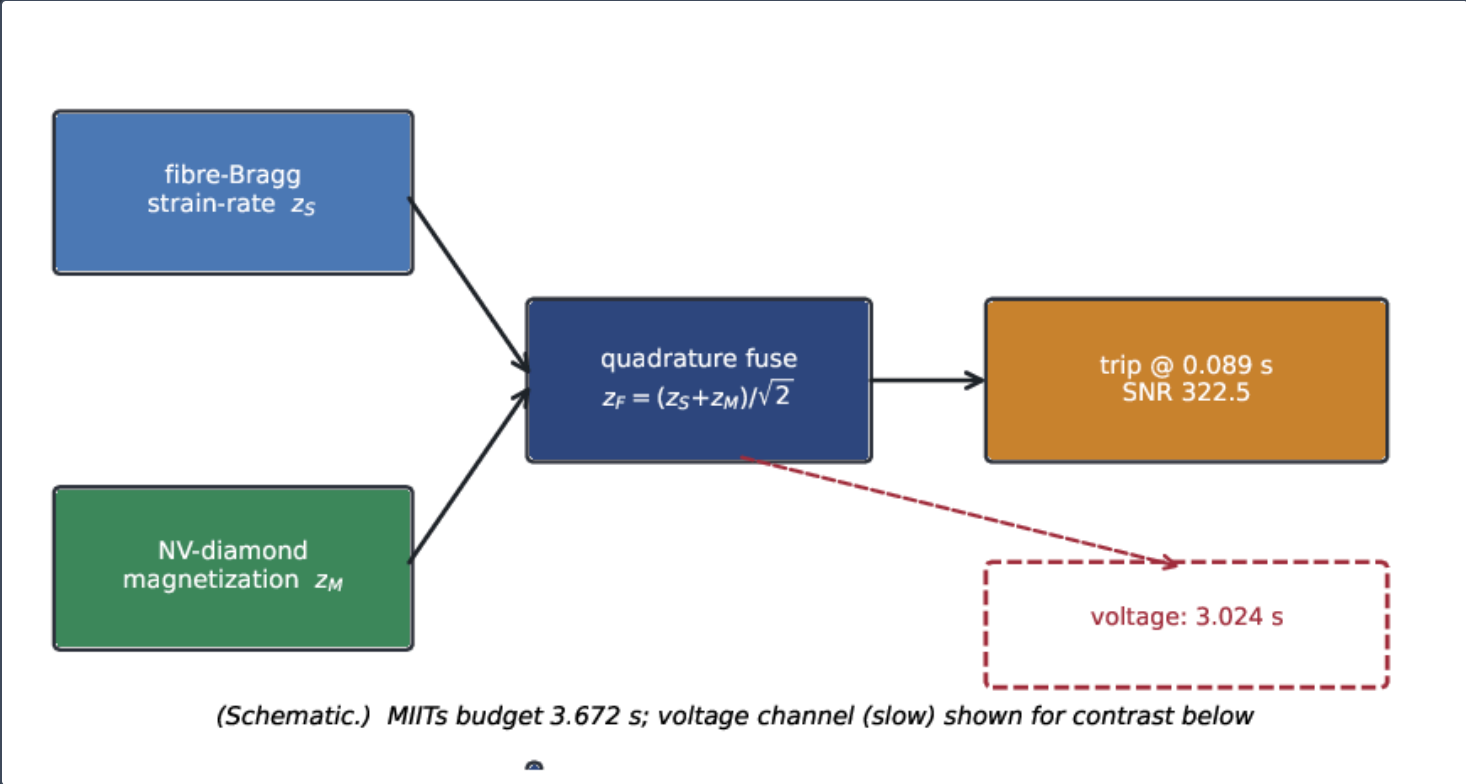
(Schematic.) The fused quench-detection architecture: a fibre-Bragg strain-rate channel and an in-winding NV-diamond magnetization channel are combined in quadrature (equation 12) to trip at 0.089 s , far ahead of the slow voltage channel ( 3.024 s ). Structure only; the numeric labels are the frozen detection results.
