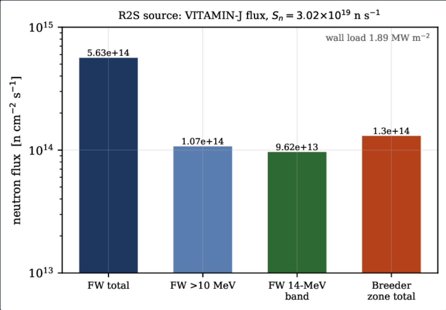
Tallied neutron flux by zone and energy band (register serial BR-L2-A23), normalized to S_n = 3.02 \times 10^{19} at P_{\text{fus}} = 85.04 MW. The 14 MeV band drives the threshold activation reactions; the breeder-zone flux is moderated below the first-wall value.
