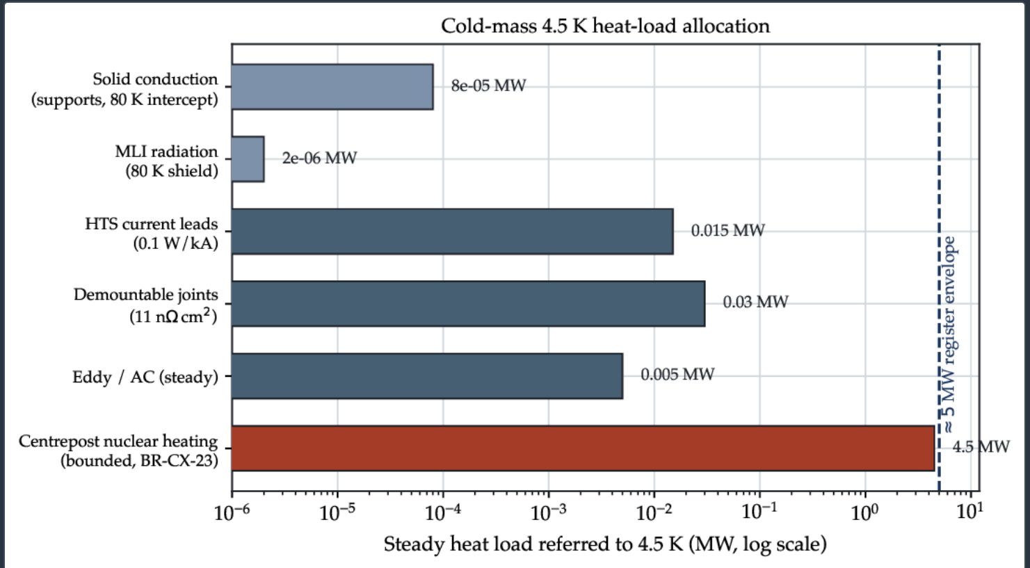
Cold-mass heat-load allocation (log scale). The classical parasitic leaks close to < 0.1 \text{ MW} ; centrepost nuclear heating is the register-bounded, three-dimensionally-queued dominant term (BR-CX-23). The dashed line marks the \approx 5 \text{ MW} register envelope.
