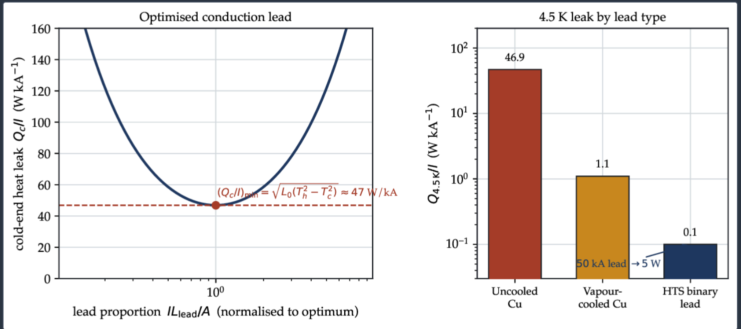
Current-lead heat leak. Left: the convex heat-leak curve of an uncooled conduction lead (Eq. 6) with the geometry-independent optimum (\dot{Q}_c/I)_{\text{min}} = \sqrt{L_0(T_h^2 - T_c^2)} \approx 47 \text{ W/kA} (Eq. 7). Right: the leak per kiloampere by lead technology; an HTS binary lead reduces the cold-end burden of a 50 kA circuit to \approx 5 \text{ W} .
