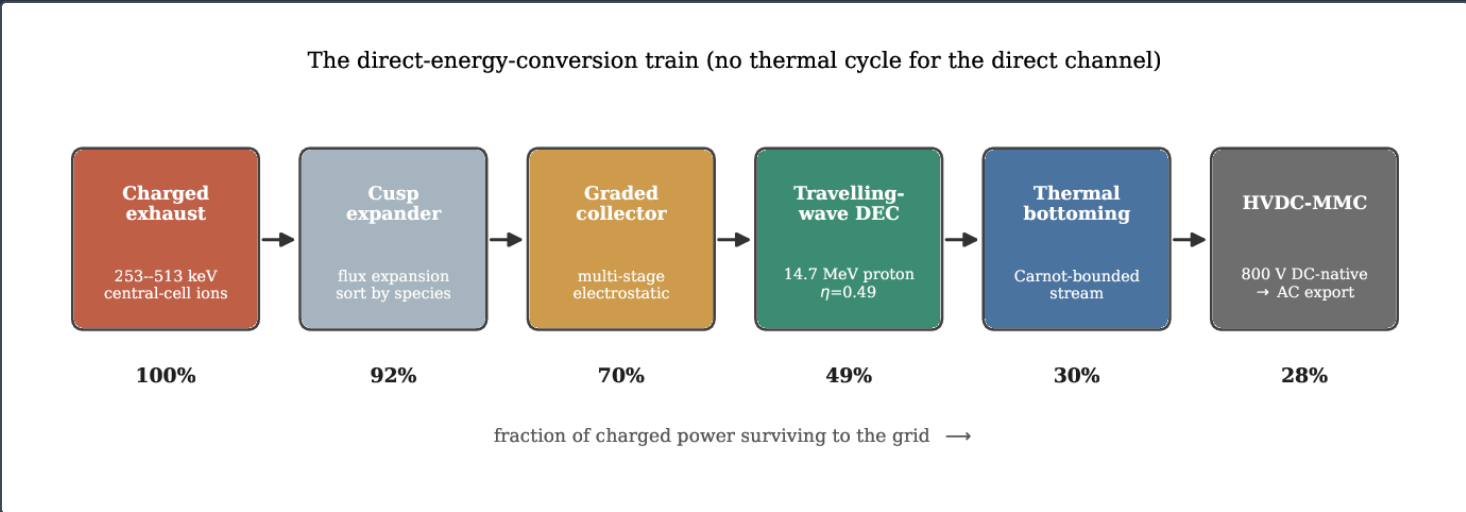
(Schematic.) The direct-energy-conversion train. Central-cell exhaust (253–513 keV) fans out in the cusp expander, is sorted by species, and is decelerated in a graded electrostatic collector; the 14.68 MeV proton channel is handled by the travelling-wave converter at the frozen anchor \eta_{\text{dec}} = 0.49 ; the Carnot-bounded remainder is recovered by a thermal bottoming cycle; the DC output is delivered HVDC-native. Fractions are illustrative of the surviving charged-power cascade, not measured stage yields.
