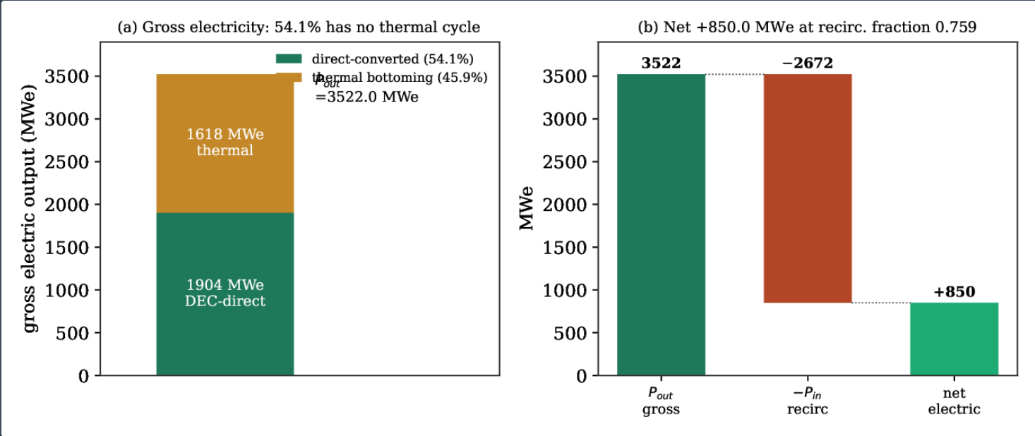
Electric power composition and net. (a) Gross electricity P_{\text{out}} = 3522.0 MWe: 54.1% direct-converted (1903.8 MWe, no thermal cycle) and 45.9% thermal bottoming (1618.2 MWe). (b) Waterfall to net: +850.0 MWe after the recirculating input P_{\text{in}} = 2672.0 MWe ( \varepsilon = 0.759 ). Register anchors (BU-L1-A10) [1] .
