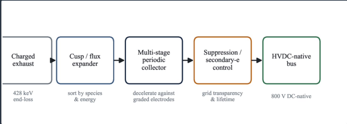
(Schematic.) The collector cascade: the 428 keV charged exhaust is expanded and sorted by species and energy, decelerated against the graded periodic collector, cleaned of back-streaming secondaries by a suppression stage, and delivered to the HVDC-native bus. No measured values are drawn.
