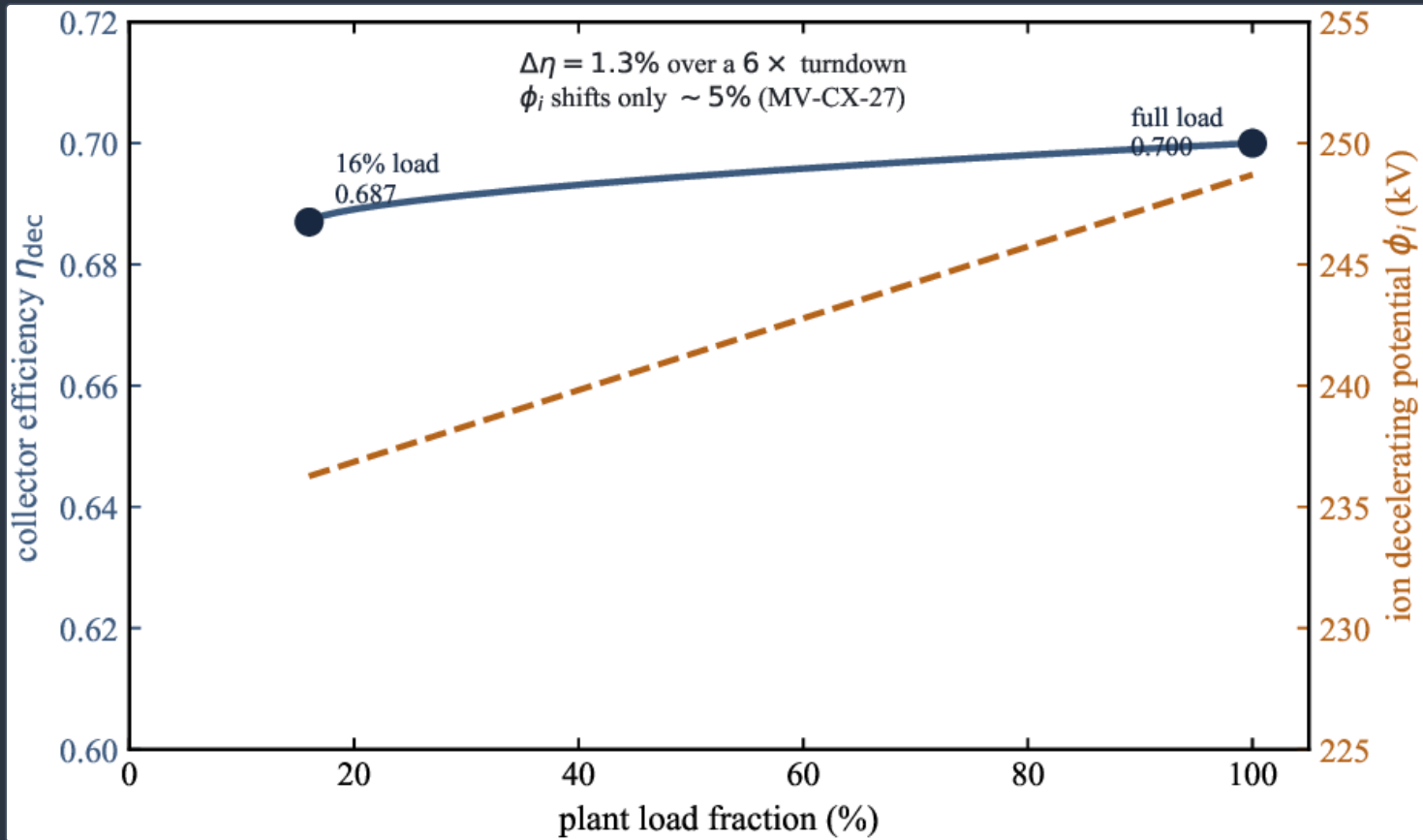
Throttling robustness. Collector efficiency (left axis) and ion decelerating potential \phi_i (right axis) versus plant load fraction. The two frozen endpoints ( 0.700 at full load, 0.687 at 16% ; MV-CX-27) bound a 1.3 -point drop over a 6 \times turndown; \phi_i moves only \sim 5\% .
