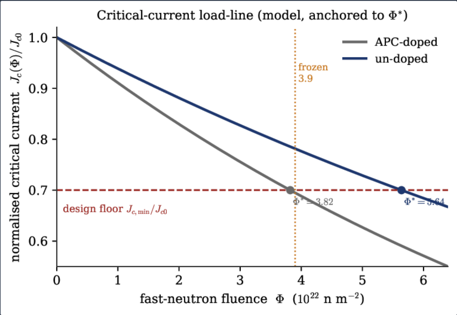
Normalised critical-current load-line J_c(\Phi)/J_{c0} from the pinning model 11, calibrated to reach the design floor J_{c, \text{min}}/J_{c0} at each grade's break-even fluence (markers). The model curve is anchored to the two frozen \Phi^* endpoints of Table 1; the un-doped grade crosses the floor at a 48 % higher fluence than the APC grade.
