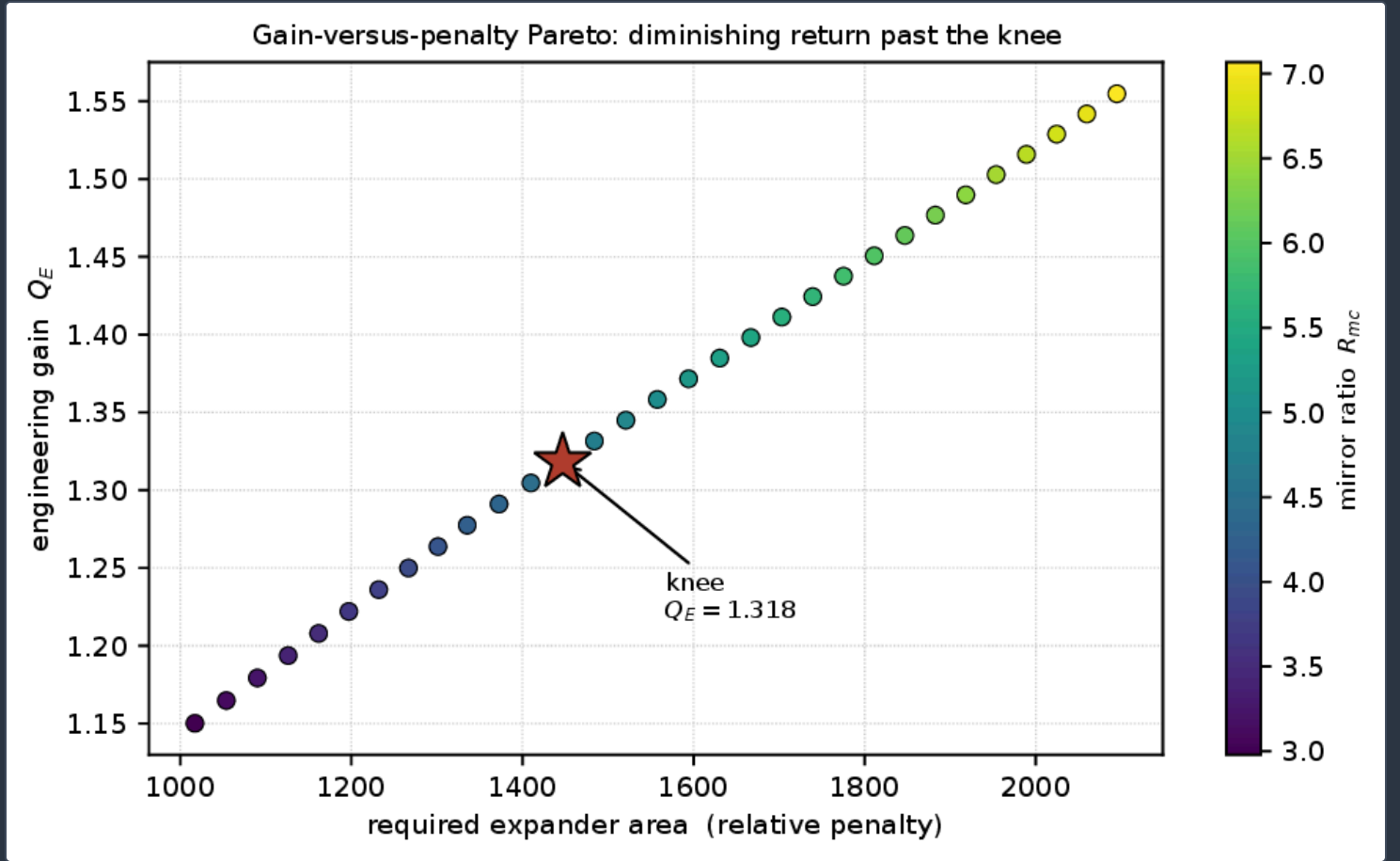
Gain-versus-penalty Pareto (AG-CX-06). Engineering gain Q_E against the relative expander-area penalty, coloured by mirror ratio R_{mc} ; the design knee ( Q_E = 1.318 ) is the red star. Gain rises with diminishing return against a penalty that grows without saturating.
