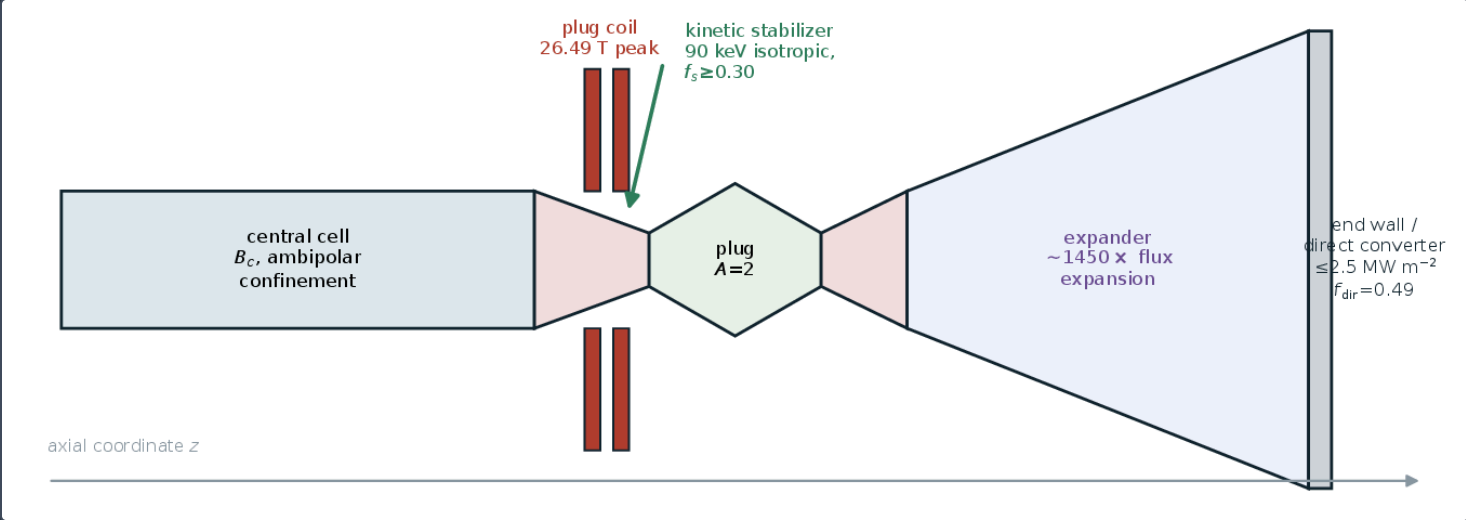
(Schematic.) End-cell layout of the Aegis burner. The central cell (field B_c , ambipolar confinement) terminates in a mirror throat and plug ( A = 2 ) behind a plug coil of 26.49 T peak conductor field; an energetic 90 keV isotropic kinetic stabilizer at f_s \geq 0.30 holds the plug micro-stable; the surviving flux tube fans out through a \sim 1450\times expander onto the end wall / direct converter at the 2.5 MW m -2 limit with direct-conversion fraction 0.49 . No data values are plotted; the figure encodes structure only.
