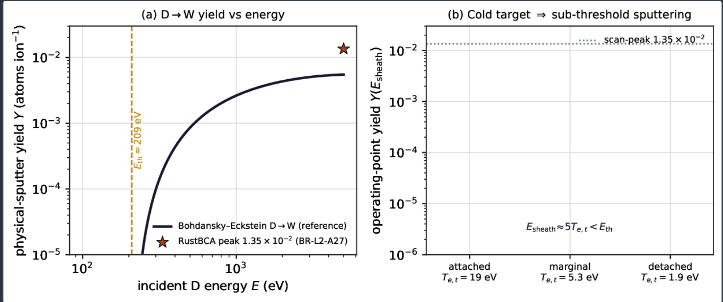
Target sputtering (register BR-L2-A27). (a) Deuterium-on-tungsten physical-sputter yield versus energy: the Bohdansky–Eckstein reference curve anchored to the RustBCA scan peak 1.35 \times 10^{-2} atoms ion -1 , with the E_{th} \approx 209 \text{ eV} threshold. (b) Operating-point yield at the sheath energy E_i \approx 5T_{e,t} : the cold detached target sits below threshold, collapsing the yield.
