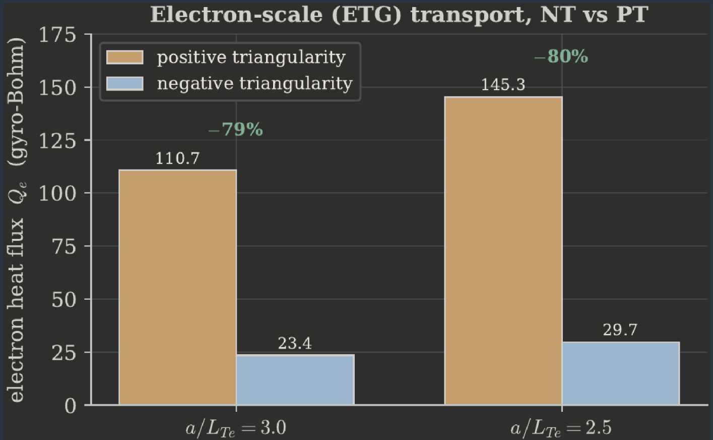
FIGURE 2. Negative triangularity suppresses turbulent transport at both the ion and electron scale relative to a positive-triangularity twin. NONLINEAR CGYRO
