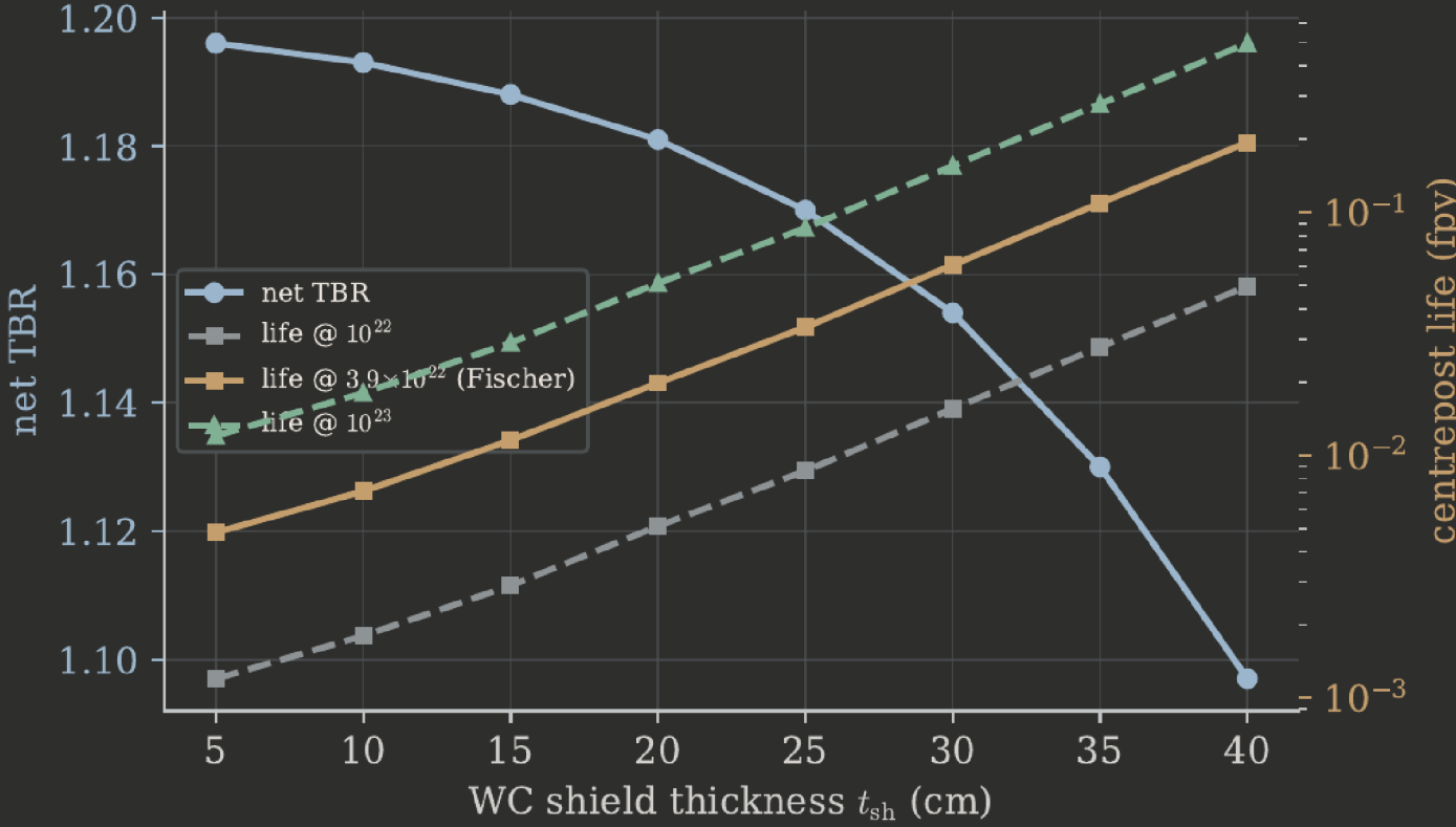
Centrepost coverage-vs-protection trade (three fluence thresholds)
