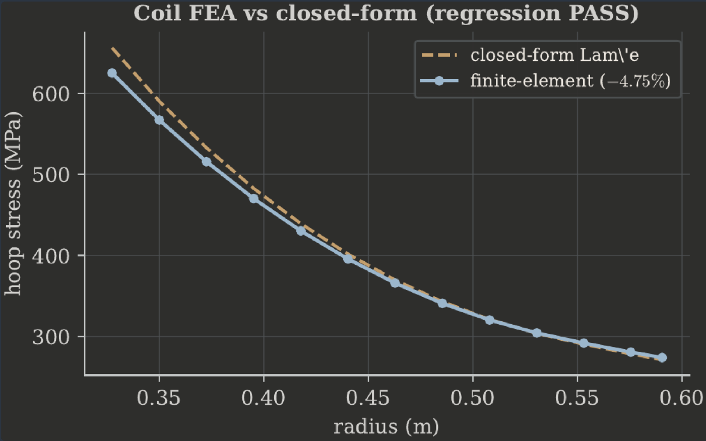
FIGURE 2. Coil structural finite-element stress against the analytic Lamé solution. RECOMPUTED
