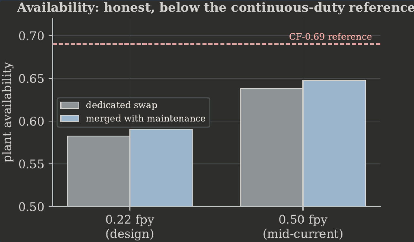
FIGURE 3. The maintenance-cadence / availability model that turns the swap into a scheduled line item. RECOMPUTED
