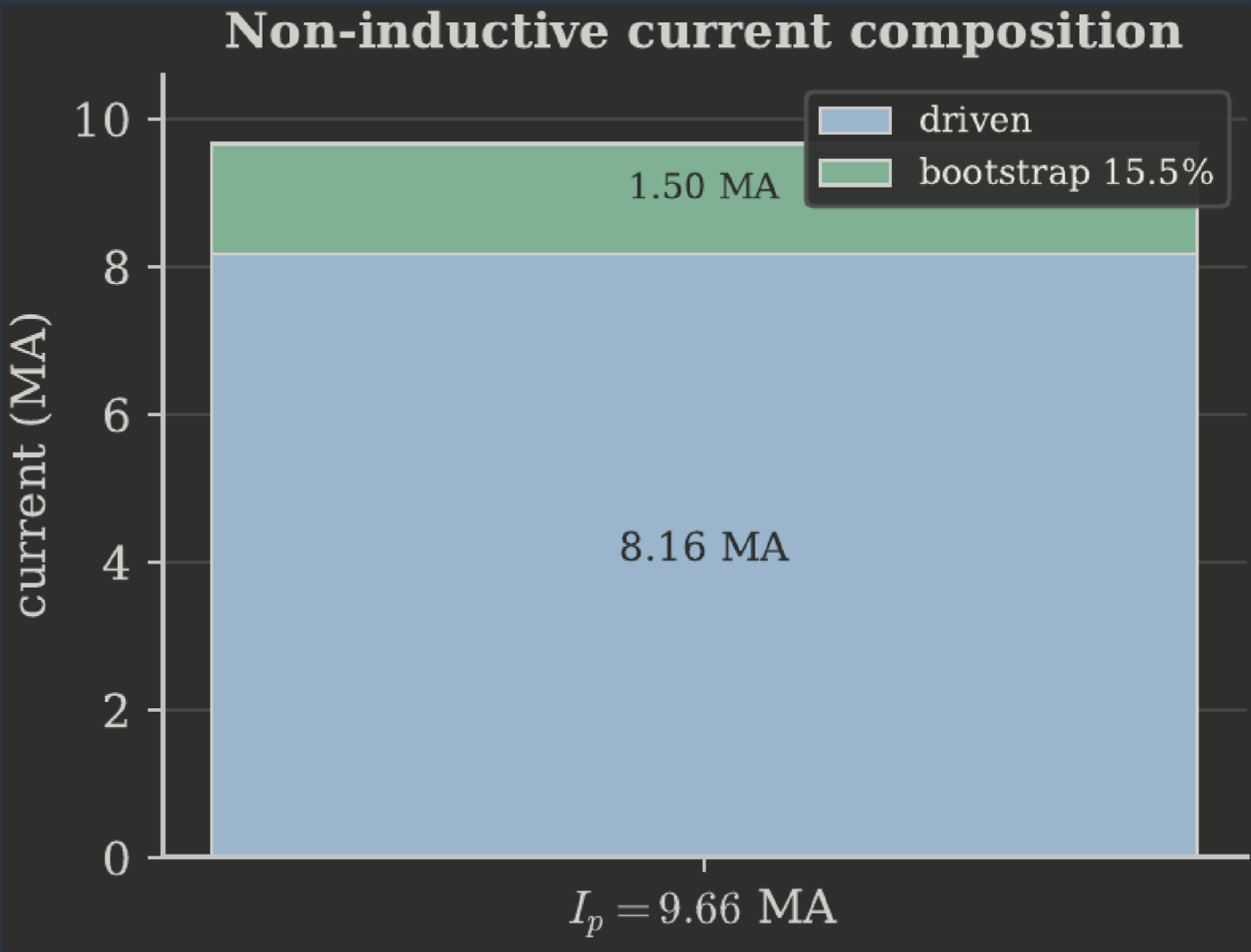
FIGURE 1. Non-inductive current composition: bootstrap and external drive of the total plasma current. DESIGN POINT
