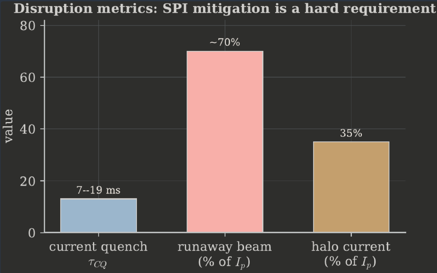
FIGURE 1. Current-quench, runaway-electron, and halo-current loads driving the mitigation requirement. NIMROD-VERIFIED
