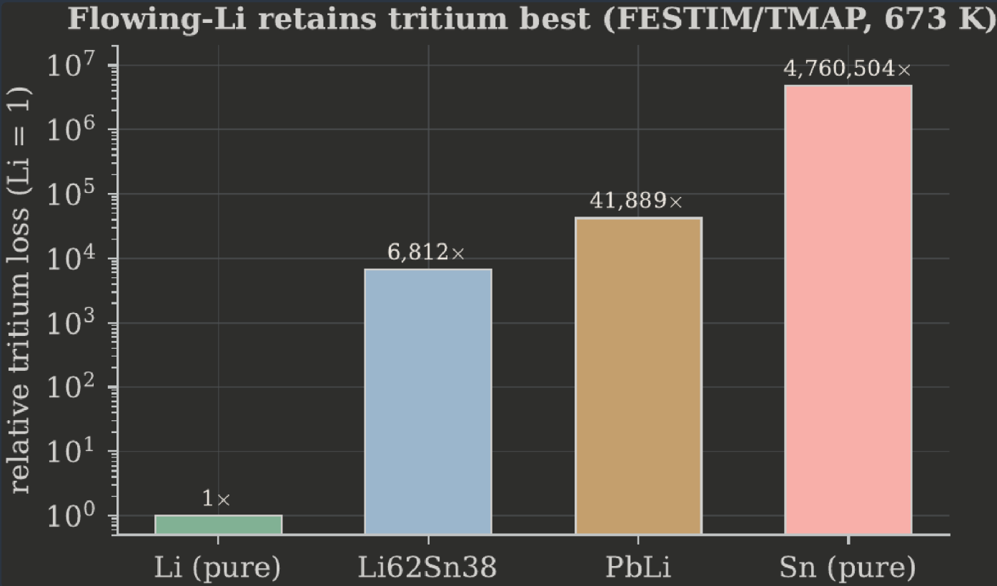
FIGURE 1. Relative tritium loss of four liquid-metal divertor candidates: flowing lithium is optimal. FESTIM/TMAP
