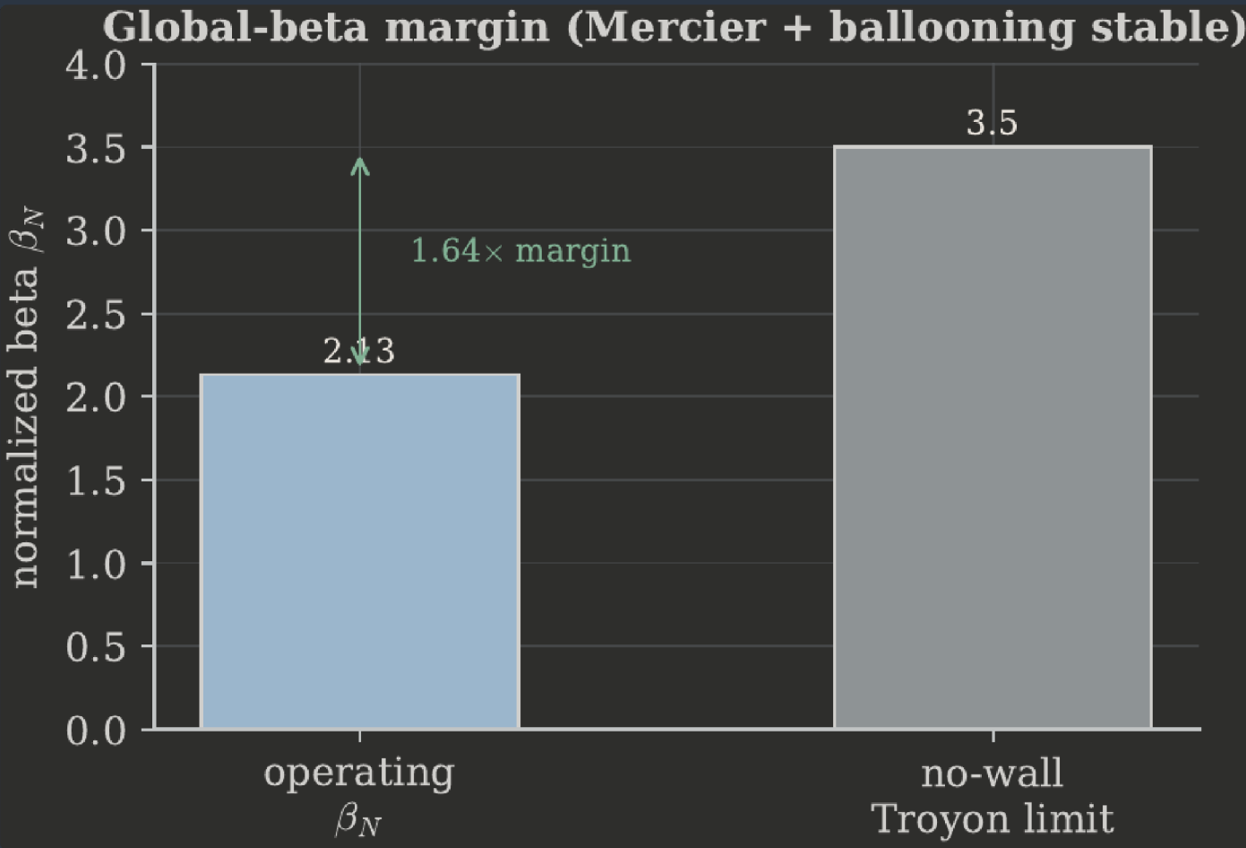
FIGURE 1. Ideal-MHD stability margins against the binding kink and ballooning limits. RECOMPUTED
