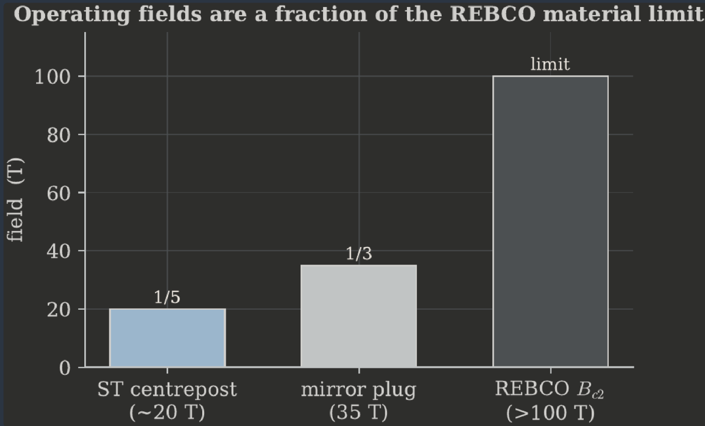
FIGURE 1. The REBCO field-capability envelope for the two machines; a conductor-capability claim, kept strictly apart from any coil record. RECOMPUTED
