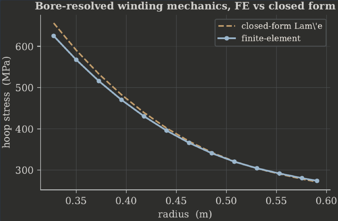
FIGURE 2. Bore-resolved hoop stress through the winding: the structural shield brings the small-bore plug coil inside its strain margin. RECOMPUTED
