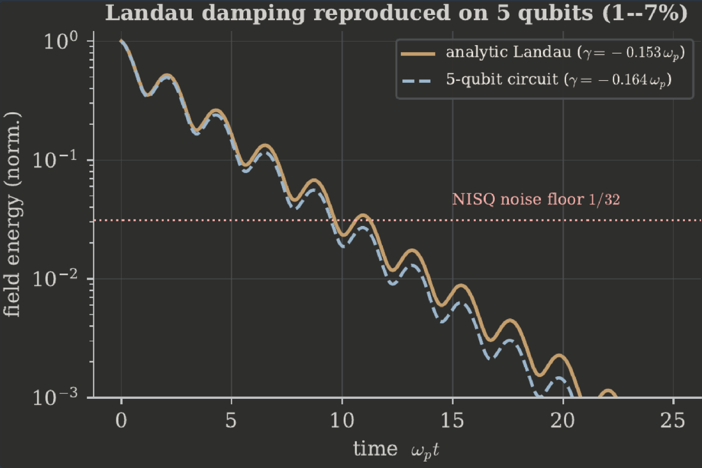
FIGURE 2. Landau damping reproduced on a 5-qubit Hamiltonian-simulation circuit. RECOMPUTED
