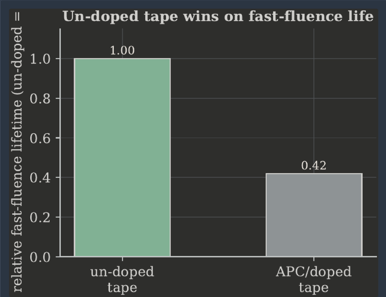
FIGURE 1. Relative fast-fluence lifetime: un-doped tape outlasts the doped tape (gates #33/46/66/68). SCREENING
