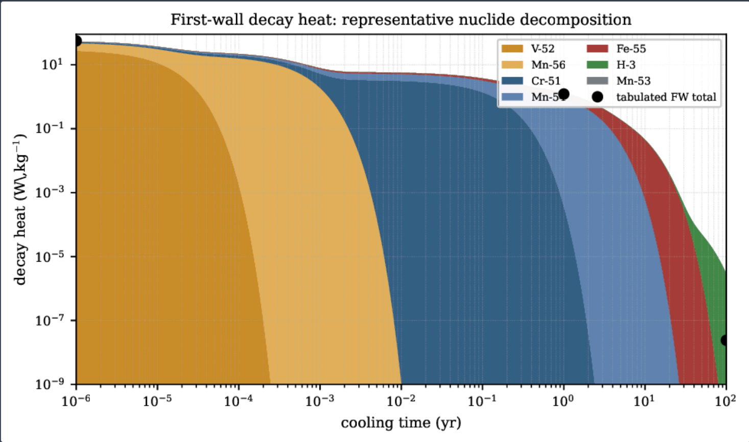
First-wall decay heat resolved into a representative nuclide-by-nuclide decomposition using the identified dominant contributors and their tabulated half-lives, normalised so the stacked total tracks the tabulated first-wall anchors (black markers). 56 Mn/ 52 V dominate at shutdown, 51 Cr/ 54 Mn/ 55 Fe through the first year, and a 3 H/ 53 Mn residue remains at a century. (Representative decomposition consistent with the identified nuclides; totals are the tallied values.)
