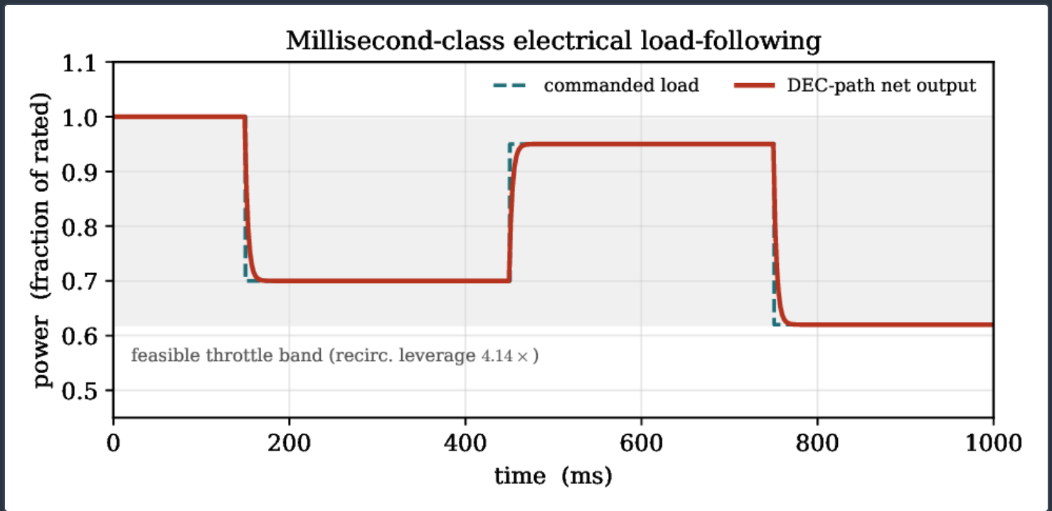
Millisecond-class electrical load-following (BU-007, MV-L1-A1). The DEC-path net output tracks a commanded-load staircase with an actuator time constant of a few milliseconds; the feasible net band is bounded below by the 4.14x recirculation leverage (shaded). Load values are fractions of rated output.
